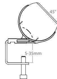
PCC - polar C clamp bracket (5-35mm)
