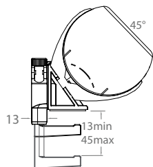
TRA - Tool rail/Panel fixing* adaptor
