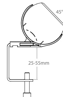
XCC - polar extended clamp bracket (25-55mm)
